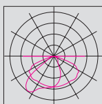
STREAM LED
